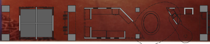
INTERIOR FLOORPLAN - WEST WALL OF CONFERENCE SPINE - SECOND FLOOR
